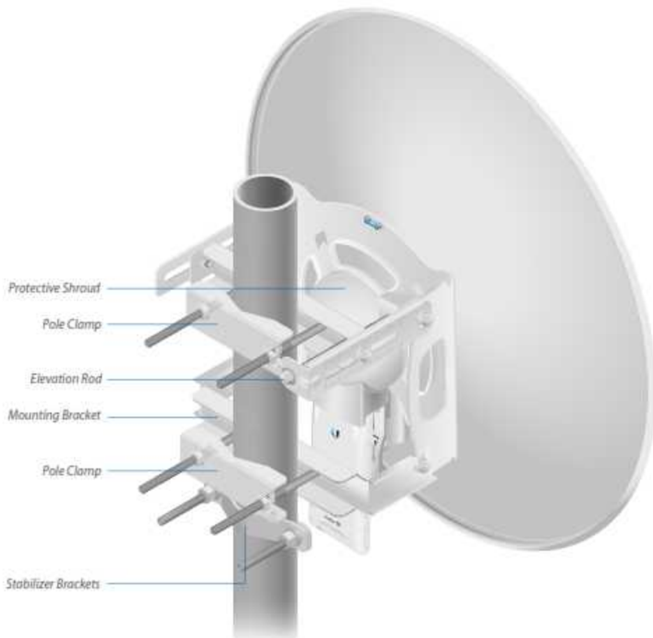
Back View of the Fully Assembled RD-5G30-LW
