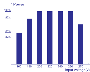
Loading capability diagram
