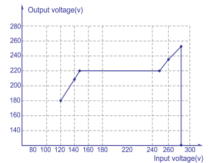
Input/output voltage diagram
